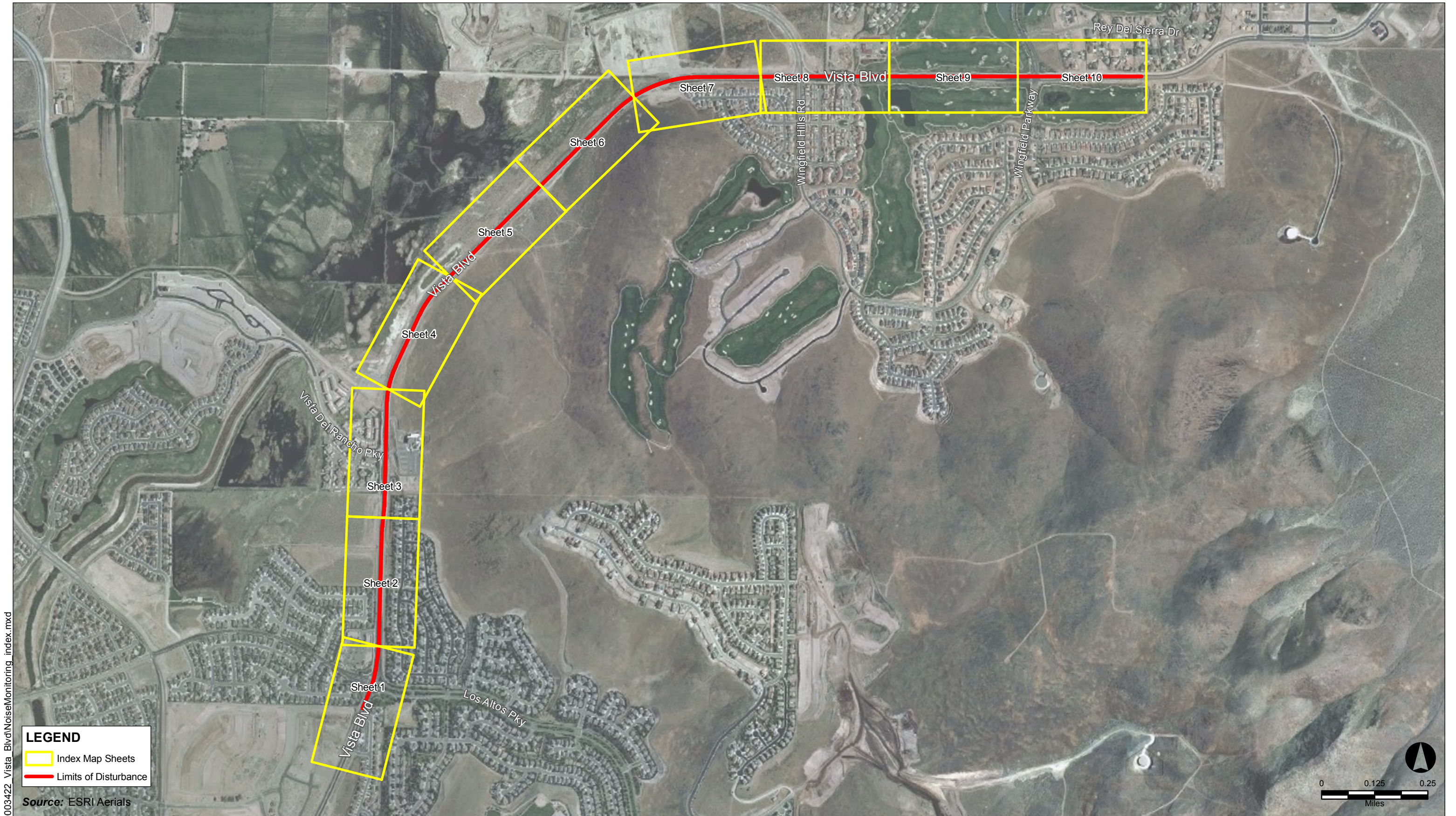
FIGURE 2 Noise Monitoring Locations and Soundwalls - Index Map
