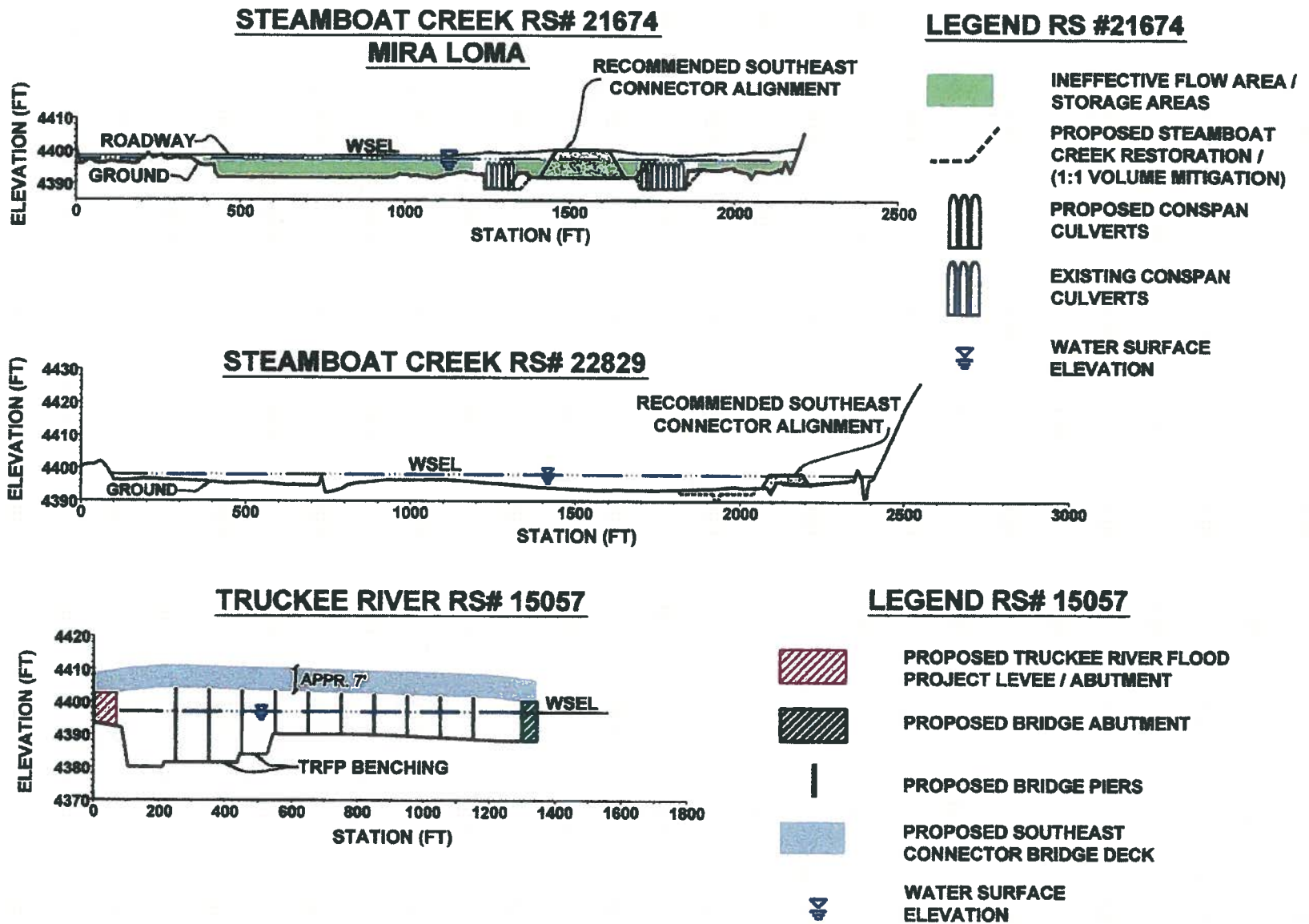
FIGURE 5 SOUTHEAST CONNECTOR DRAINAGE CROSS SECTION / STORAGE AREAS
