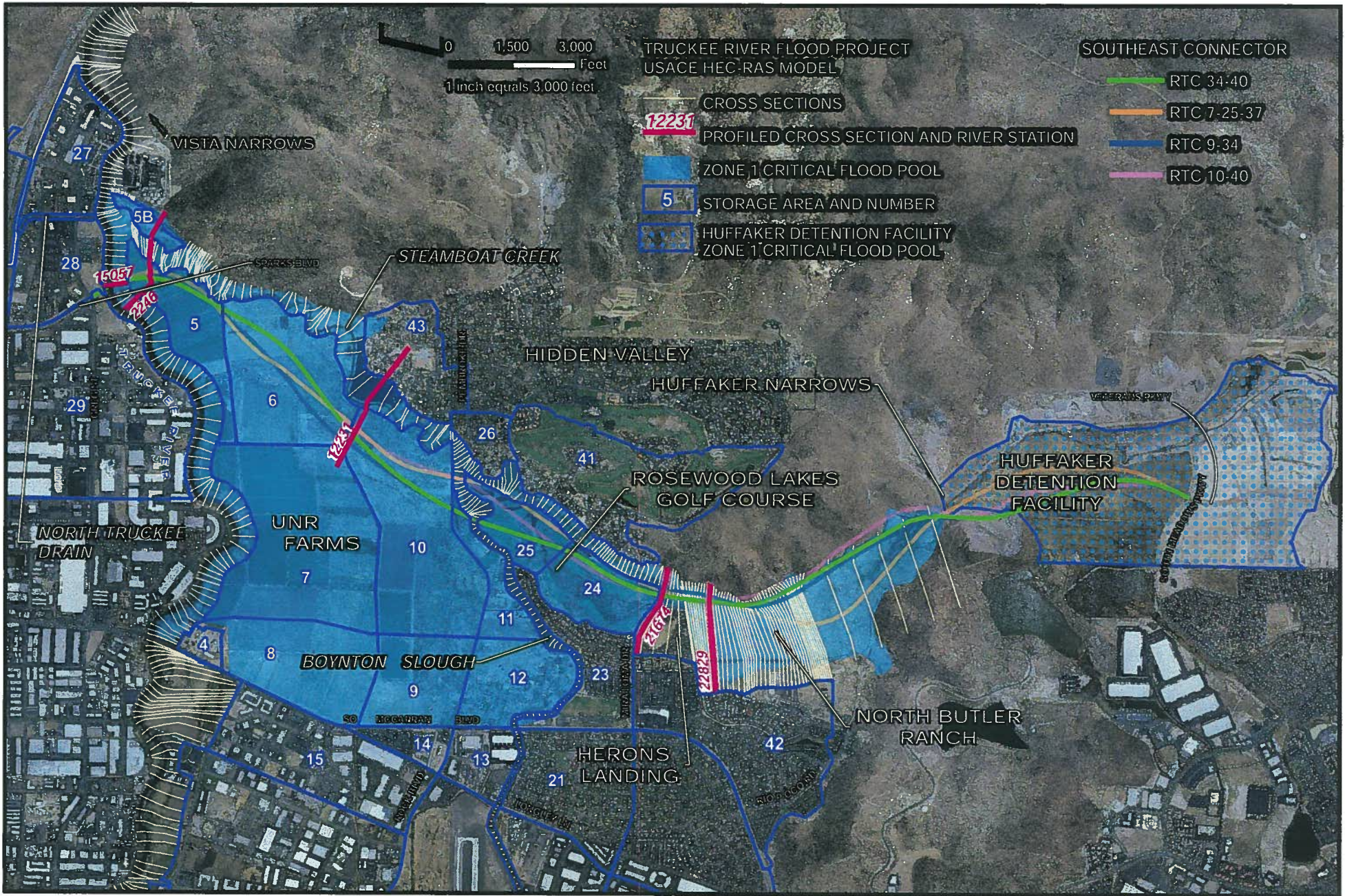
FIGURE 2 SOUTHEAST CONNECTOR DRAINAGE AND FLOOD CONTROL MODELING
