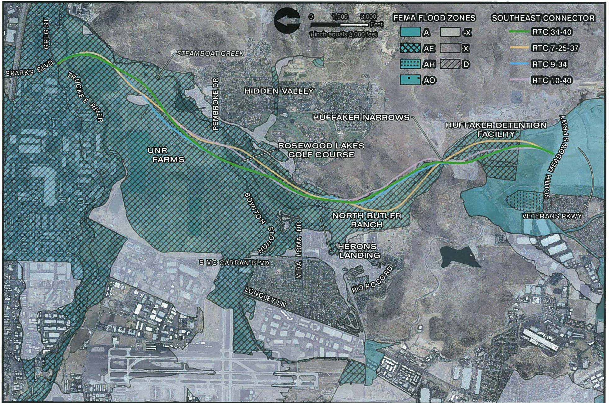
FIGURE 1 SOUTHEAST CONNECTOR FEMA FLOOD MAP
