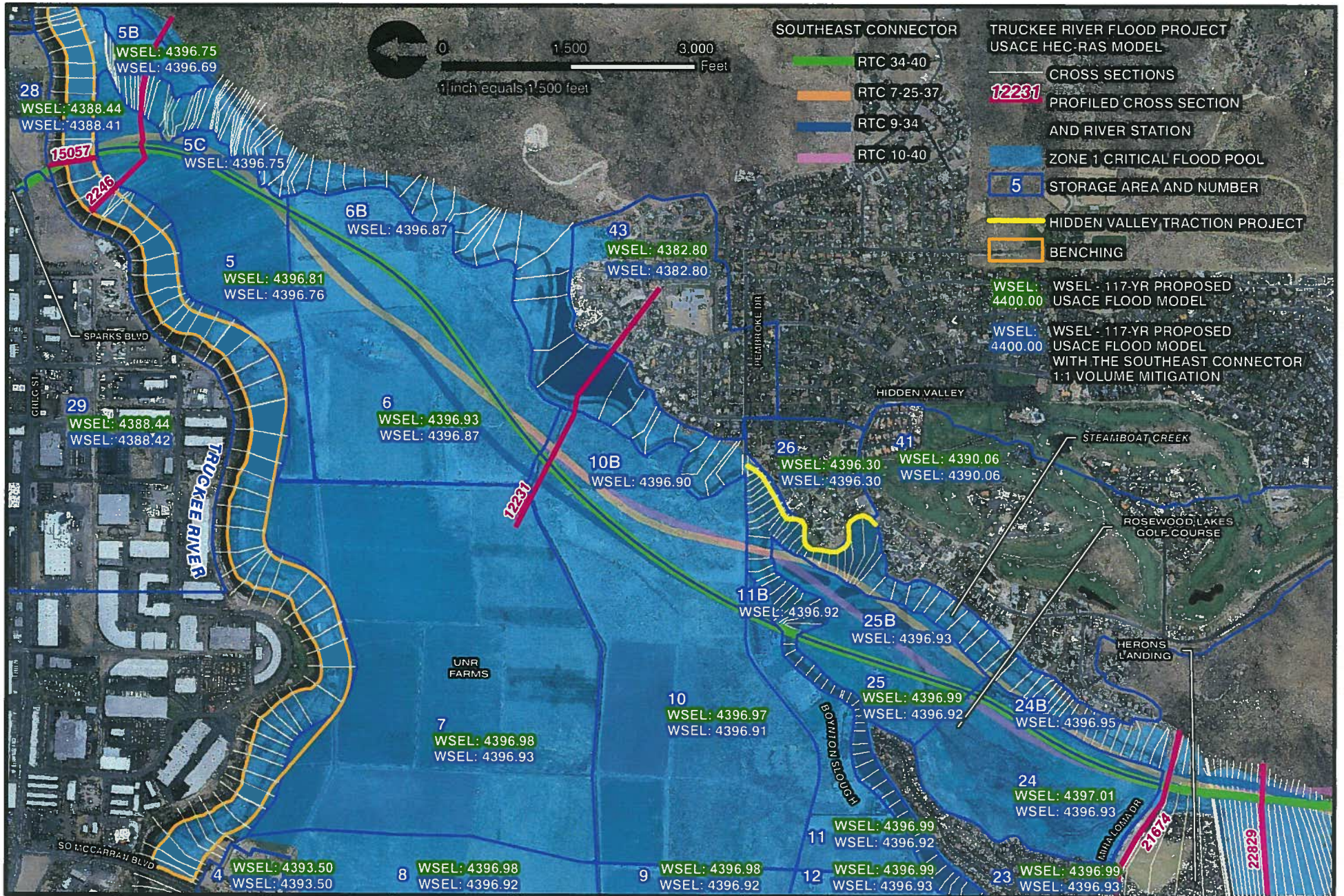
FIGURE 3 SOUTHEAST CONNECTOR DRAINAGE AND FLOOD CONTROL MODELING - SPARKS BLVD. TO MIRA LOMA DRIVE
